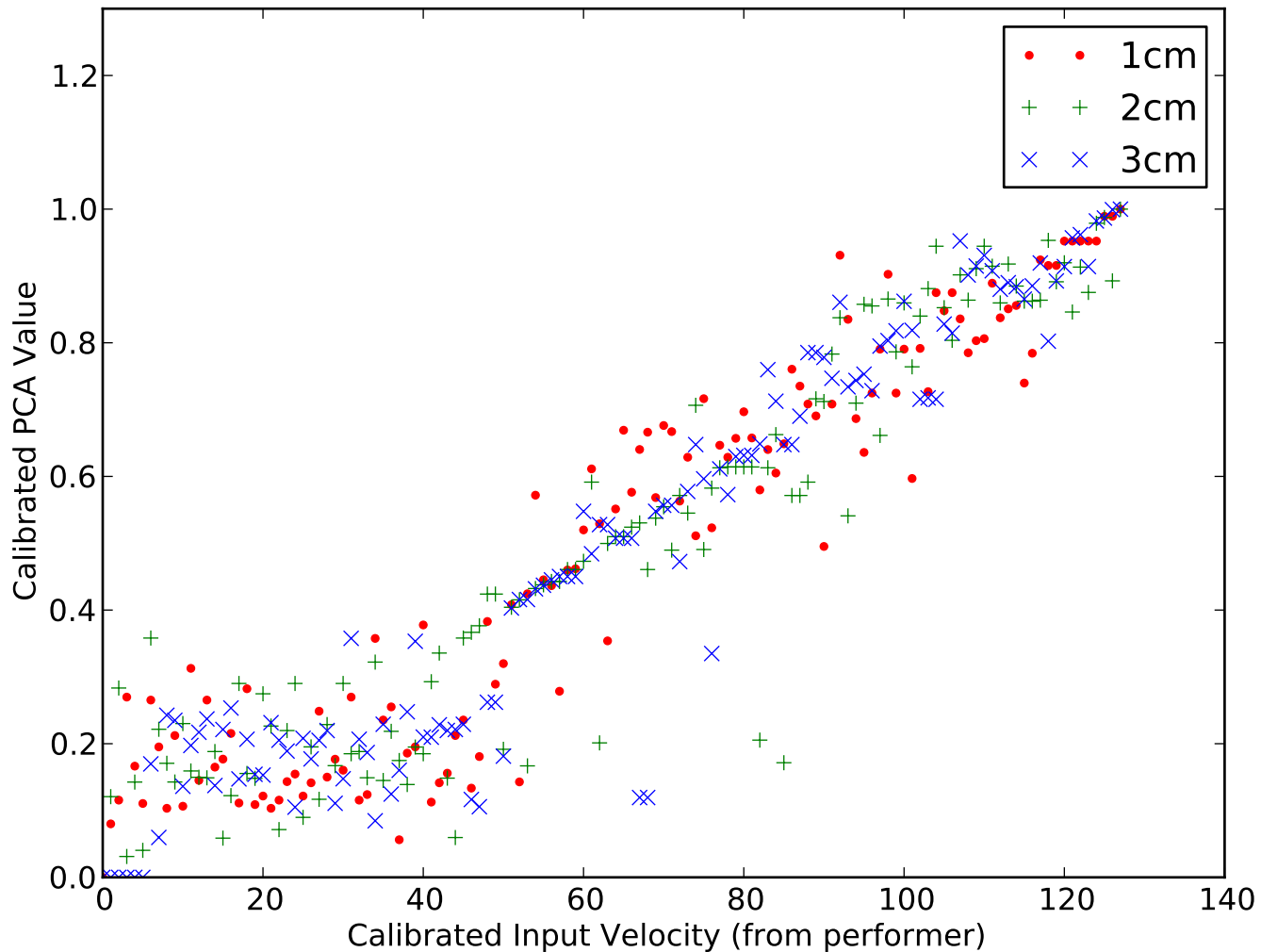
Calibrated PCA value corresponding to input velocity
